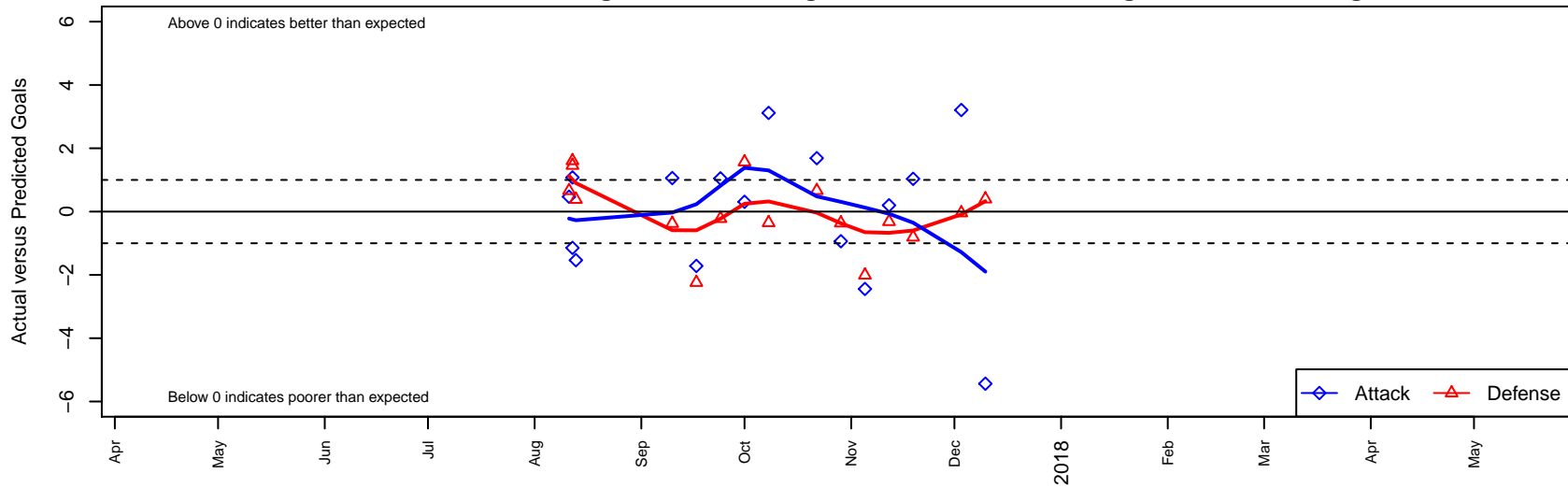
South Whidbey Wild B99 Dots are actual minus expected GF (blue circles) and GA (red triangles). Blue line is smoothed change in attack strength. Red is smoothed change in defense strength.
